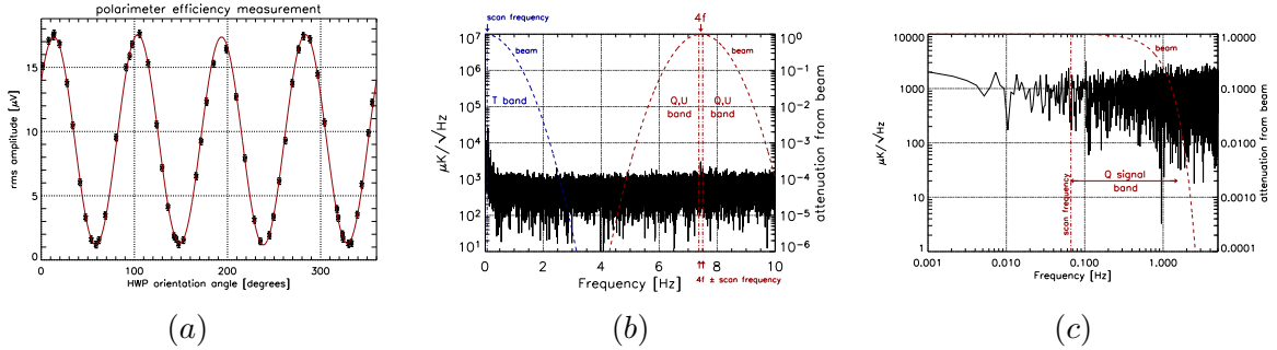
Figure 2: MAXIPOL polarimeter data from a typical photometer. (a) Results from the pre-flight characterization of the polarimeter. (b) The power spectrum of 16 minutes of time-ordered flight data with the known systematic errors corrected. (c) The power spectrum of the demodulated time ordered polarization data for Q . Zero-frequency in (c) is 4f in (b). Sky signals appear in sidebands bounded by the dashed lines marking the telescope scan frequency and the frequency-domain representation of the telescope beam in panels (b) and (c). Nominal instrument noise is recovered in all cases.
